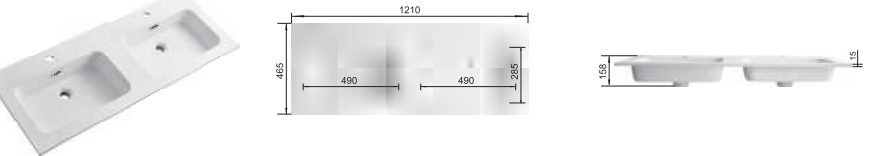
RSB1210DMW Size:1210X465X158mm
