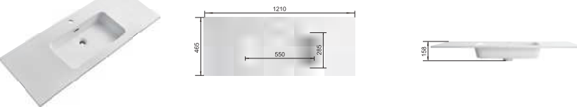
RSB1210MW Size:1210X465X158mm
