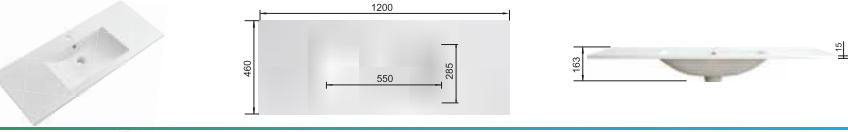
RSA1200 Size:1200X460X163mm
