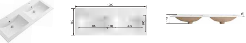
RSA1200D Size:1200X460X163mm
