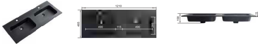
RSB1210DMB Size:1210X465X158mm
