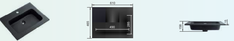
RSB610MB Size:610X465X158mm
