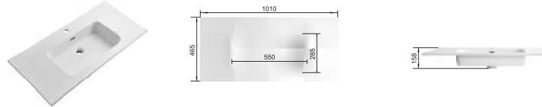
RSB1010MW Size:1010X465X158mm
