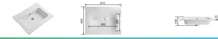
RSB610MW Size:610X465X158mm
