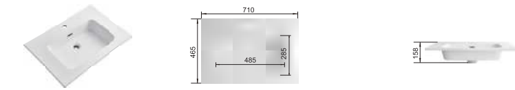
RSB710MW Size:710X465X158mm
