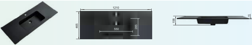
RSB1210MB Size:1210X465X158mm
