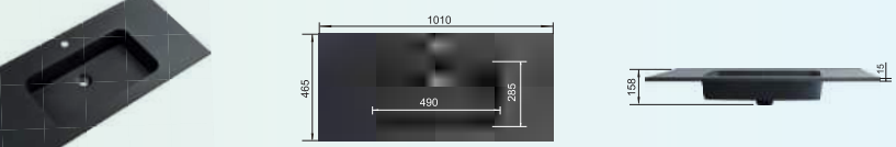
RSB1010MB Size:1010X465X158mm
