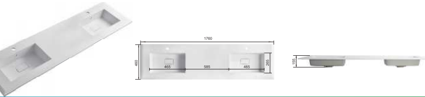
RSZ1760DMW Size:1760X460X155mm
