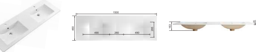
RSA1500D Size:1500X460X163mm
