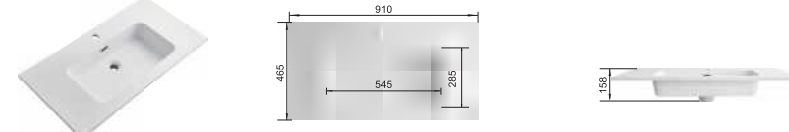
RSB910MW Size:910X465X158mm
