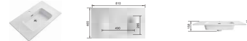
RSB810MW Size:810X465X158mm
