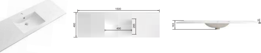
RSA1500 Size:1500X460X163mm
