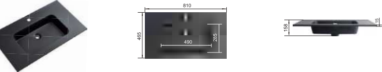
RSB810MB Size:810X465X158mm
