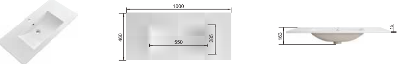
RSA1000 Size:1000X460X163mm
